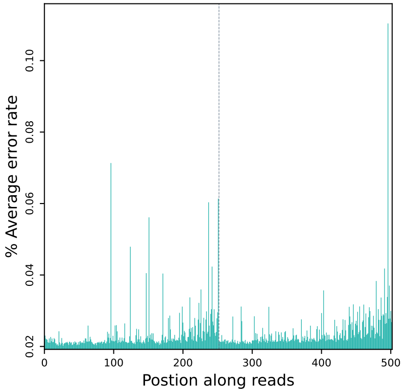
Error rate distribution along reads (R20212)
